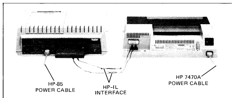
HP-IL Interface Cable Connection
