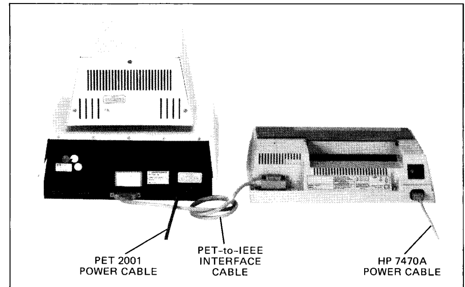
PET-to-IEEE Cable Connection
