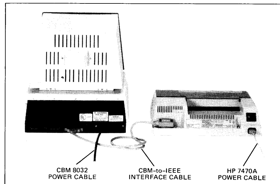
CBM-to-IEEE Cable Connection
