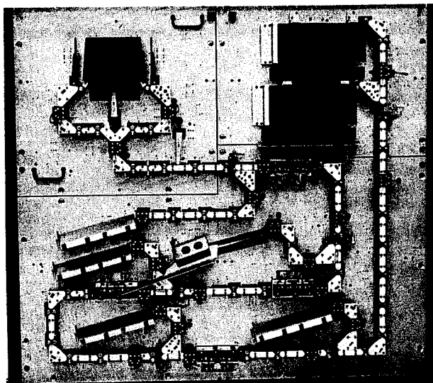
Fig. 1. To record the timing tracks and programs on the magnetic cards for the HP-75 Portable Computer, this production system was designed and built. It accepts blank cards in any possible orientation, rejects bad cards, and can record 2500 cards per hour.
