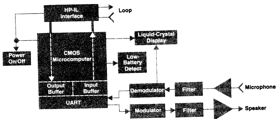
Fig. 2. Block diagram of the electronics used in the 82168A Acoustic Coupler.
