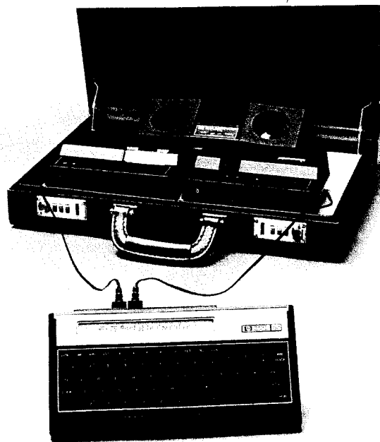
Fig. 2. This HP-75 system features HP's 82168A Acoustic Modem, 82162A Thermal Printer/Plotter, and 82161A Digital Cassette Drive.
