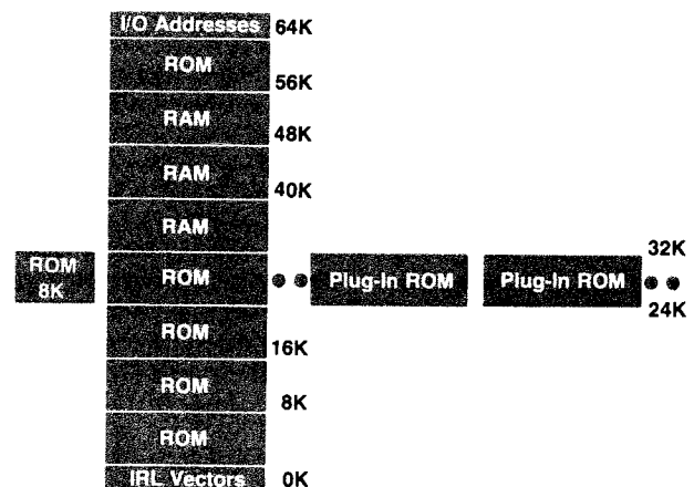
Fig. 3. Memory organization in the HP-75 Portable Computer.
