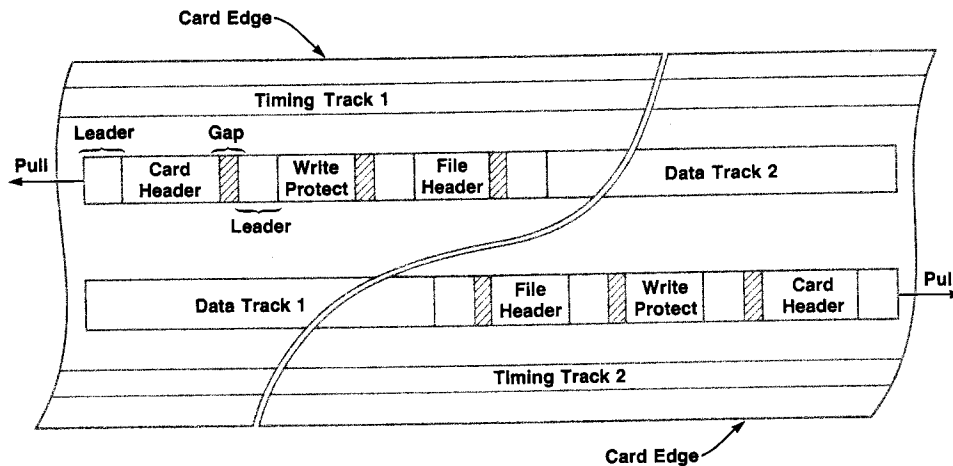
Fig. 2. Magnetic card track and data field format.
