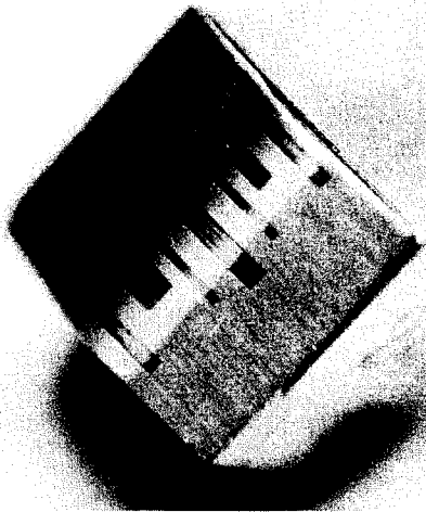
Fig. 3. A common read-after-write head design locates the read and write gaps on opposite sides of the head's crown. The head used in the HP-75 has these gaps located on the crown as shown.
