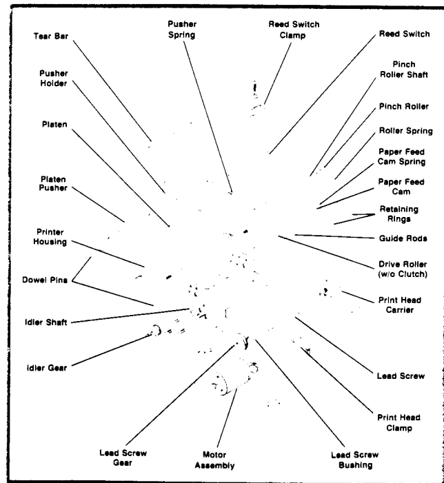
Fig. 9. Printer mechanism.
