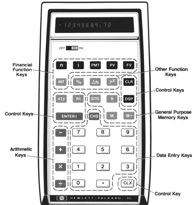
Figure 1. Keyboard Layout
