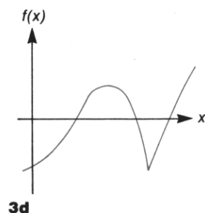
Figure B-3. Functions for Which a Root Can Be Found
